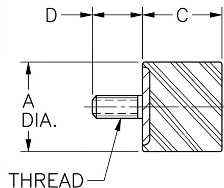
Vibration Bumper Foot
