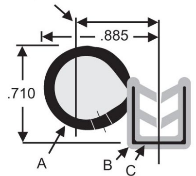
Compression Line
